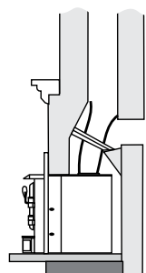
2) Direct Flue Connection with Cleanout
