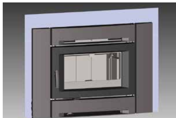
Diagram 5 Standard backing plate shown on the CI1250
